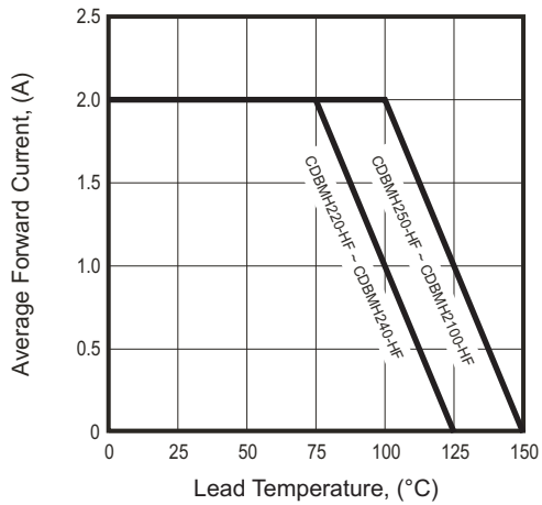
Fig.1- Typical Current Derating Curve
